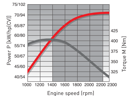
QUANTUM C POWER CURVE
